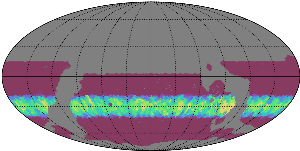
noroll_mjdp365_v3.4_10yrs WFD u band: Min normairmass
