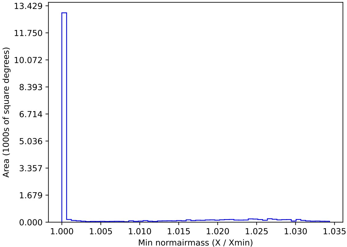
noroll_mjdp365_v3.4_10yrs WFD r band: Min normairmass
