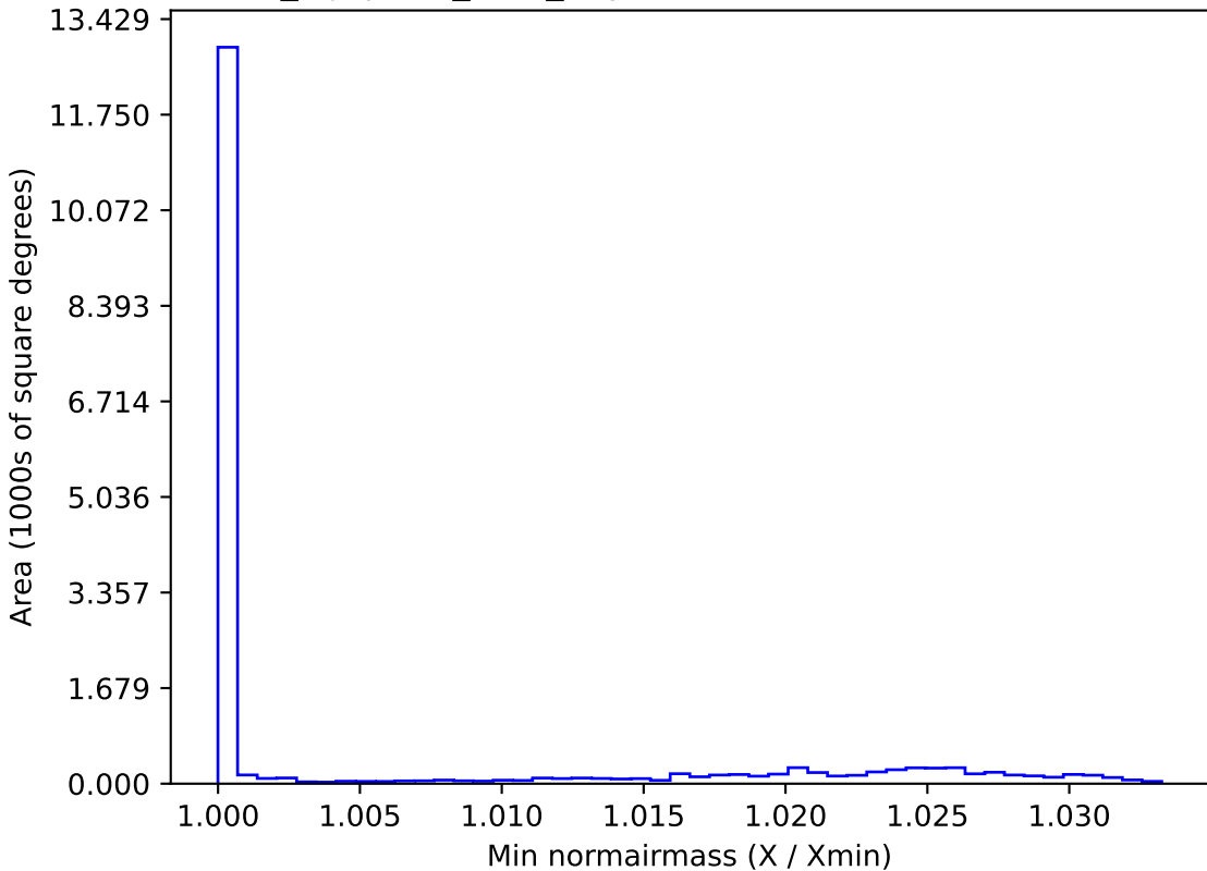
noroll_mjdp365_v3.4_10yrs WFD i band: Min normairmass
