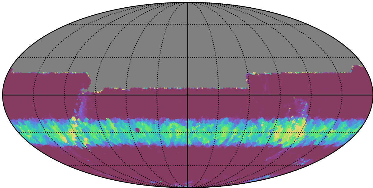
noroll_mjdp365_v3.4_10yrs All sky u band: Min normairmass
