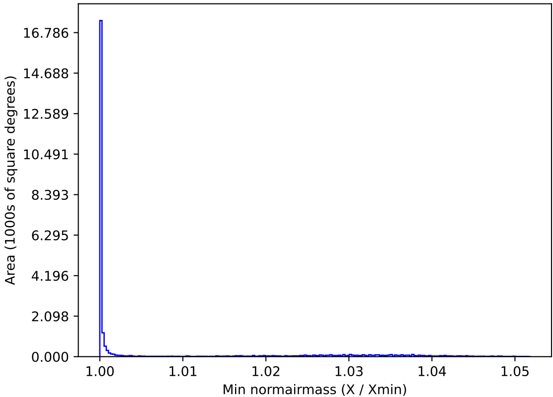
noroll_mjdp365_v3.4_10yrs All sky g band: Min normairmass
