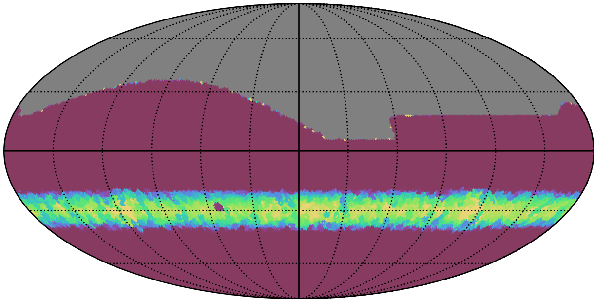
noroll_mjdp365_v3.4_10yrs All sky all bands: Min normairmass
