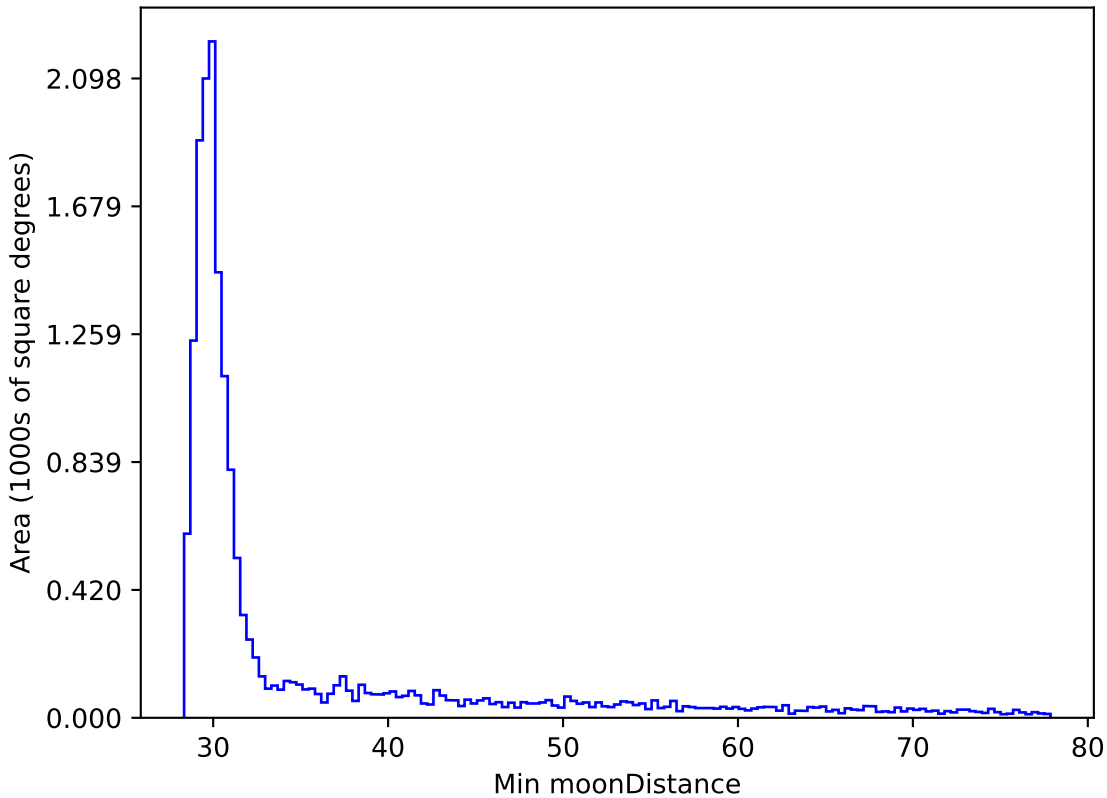
noroll_mjdp365_v3.4_10yrs WFD z band: Min moonDistance
