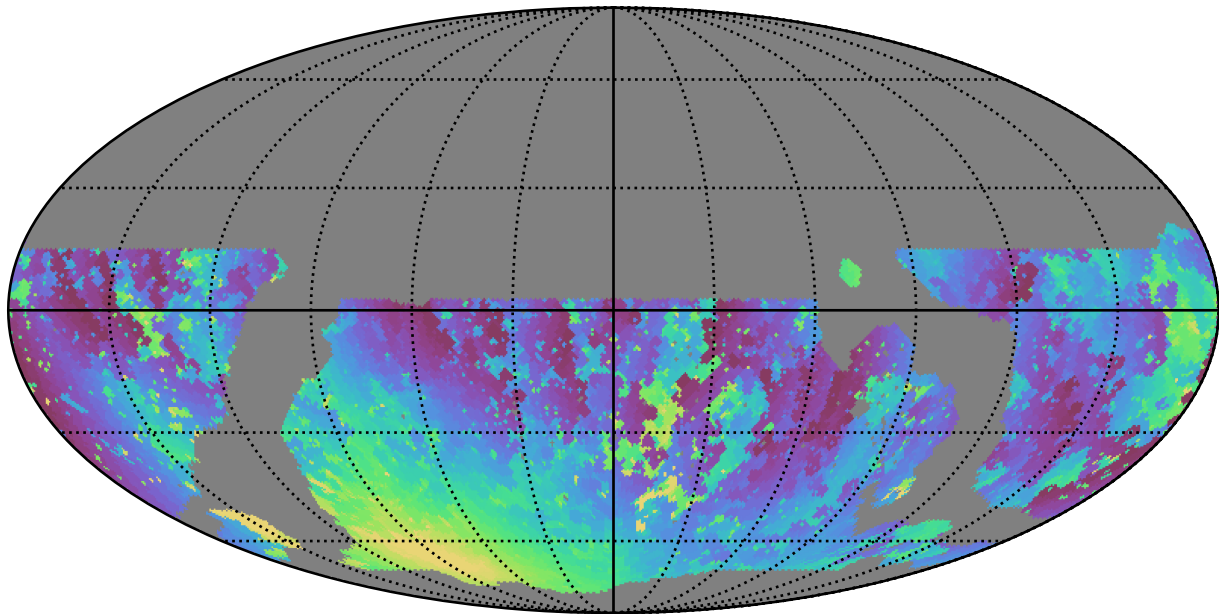
noroll_mjdp365_v3.4_10yrs WFD u band: Min moonDistance
