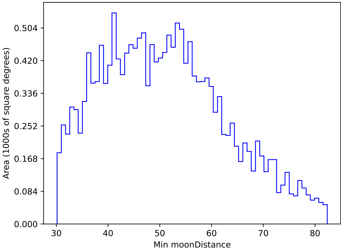
noroll_mjdp365_v3.4_10yrs WFD u band: Min moonDistance
