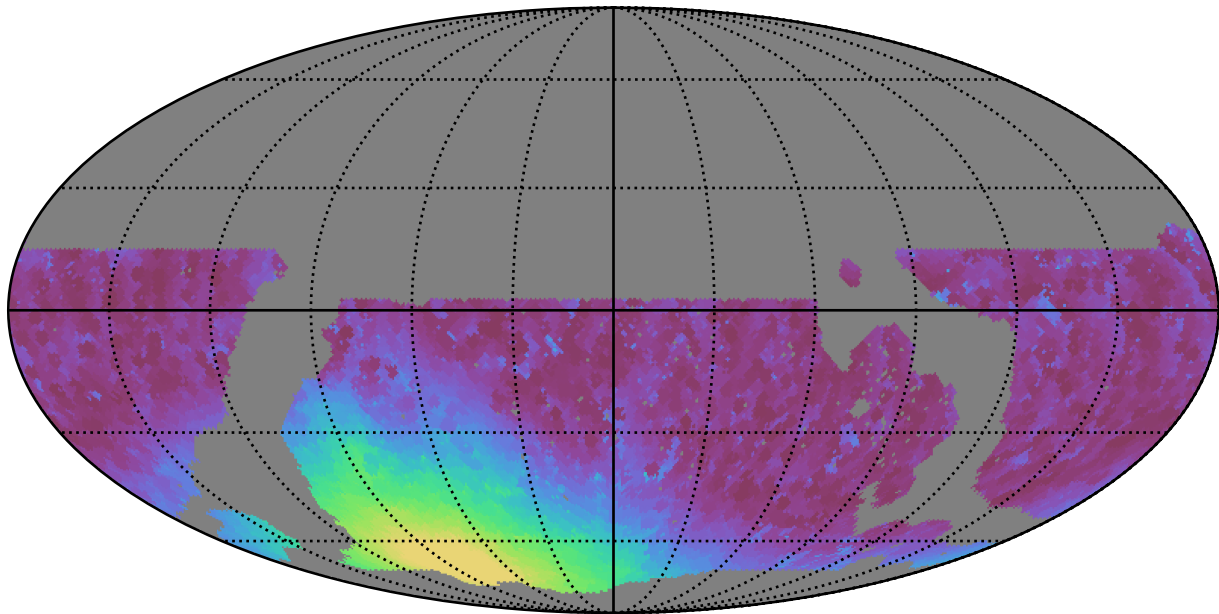
noroll_mjdp365_v3.4_10yrs WFD r band: Min moonDistance
