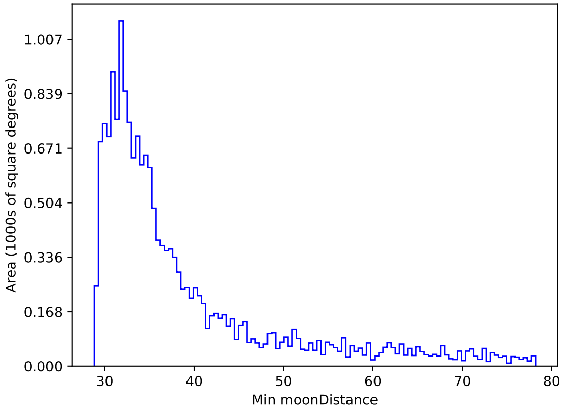
noroll_mjdp365_v3.4_10yrs WFD r band: Min moonDistance
