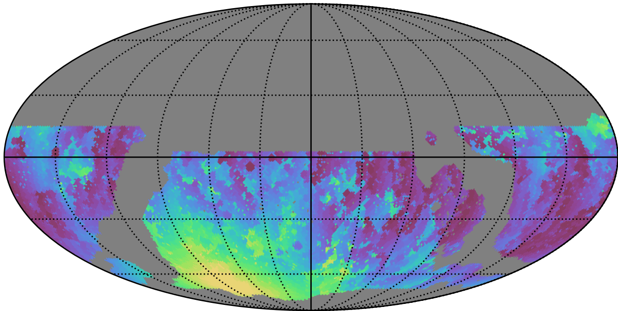
noroll_mjdp365_v3.4_10yrs WFD g band: Min moonDistance
