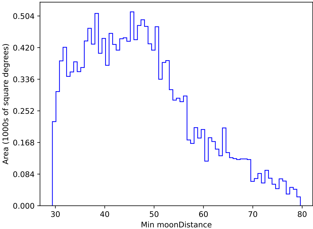
noroll_mjdp365_v3.4_10yrs WFD g band: Min moonDistance
