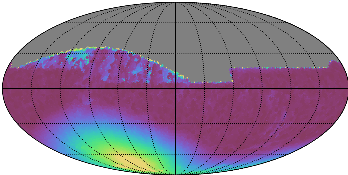
noroll_mjdp365_v3.4_10yrs All sky z band: Min moonDistance
