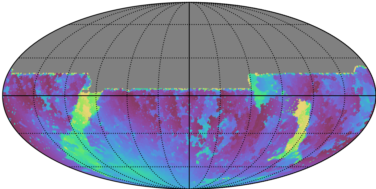
noroll_mjdp365_v3.4_10yrs All sky u band: Min moonDistance
