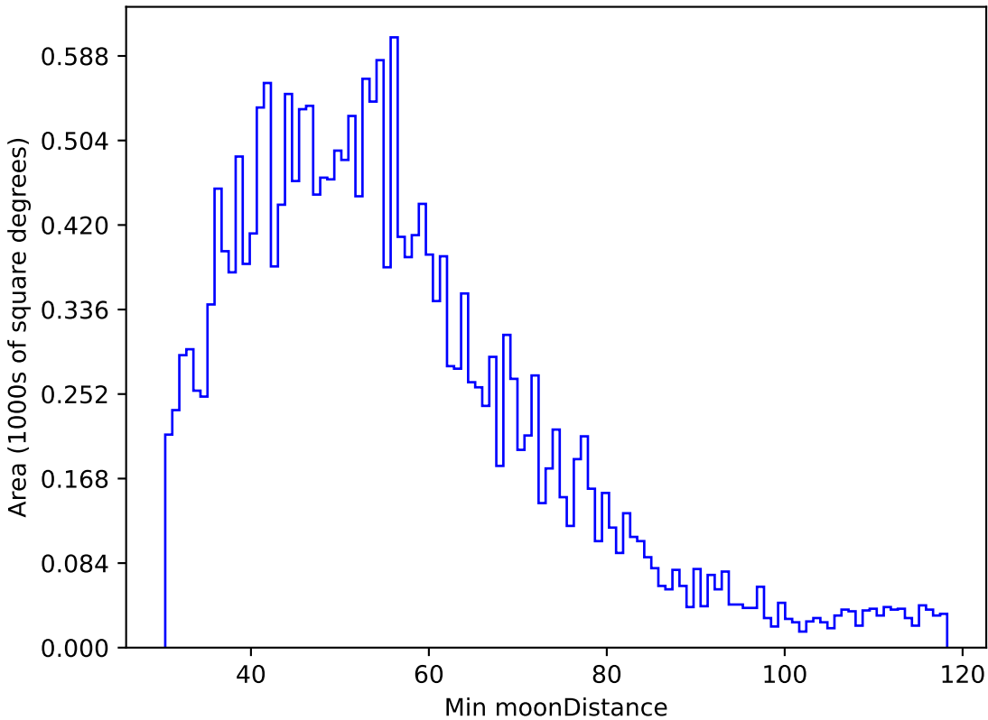
noroll_mjdp365_v3.4_10yrs All sky u band: Min moonDistance
