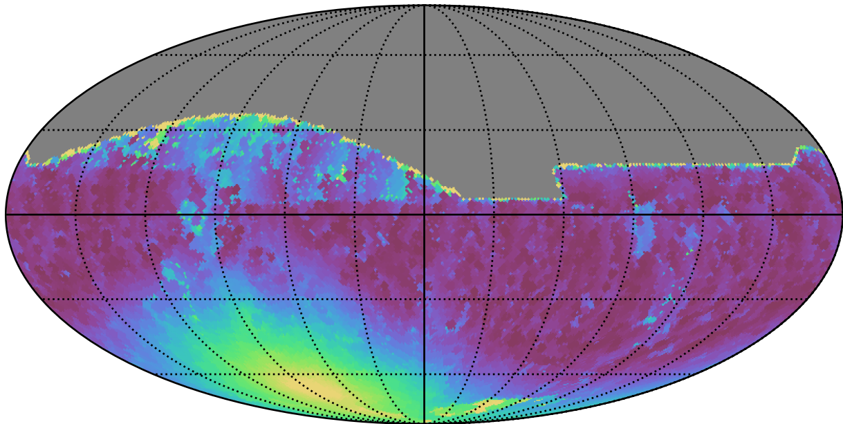
noroll_mjdp365_v3.4_10yrs All sky r band: Min moonDistance
