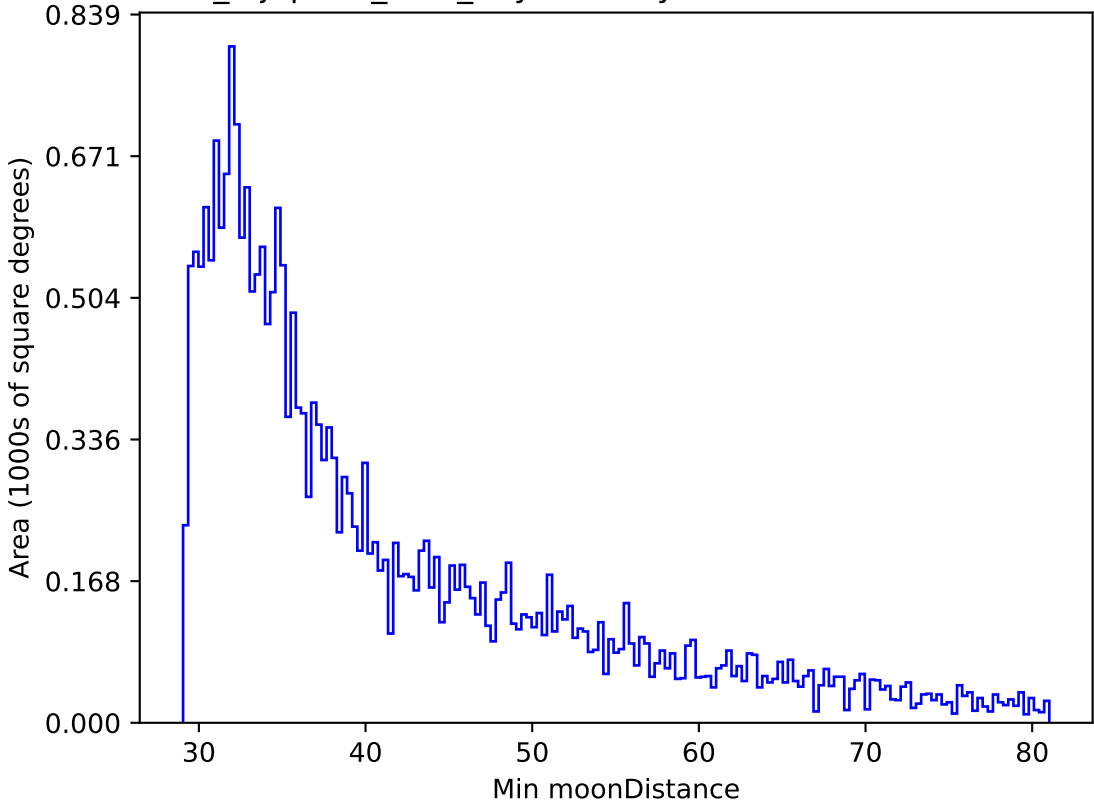
noroll_mjdp365_v3.4_10yrs All sky r band: Min moonDistance
