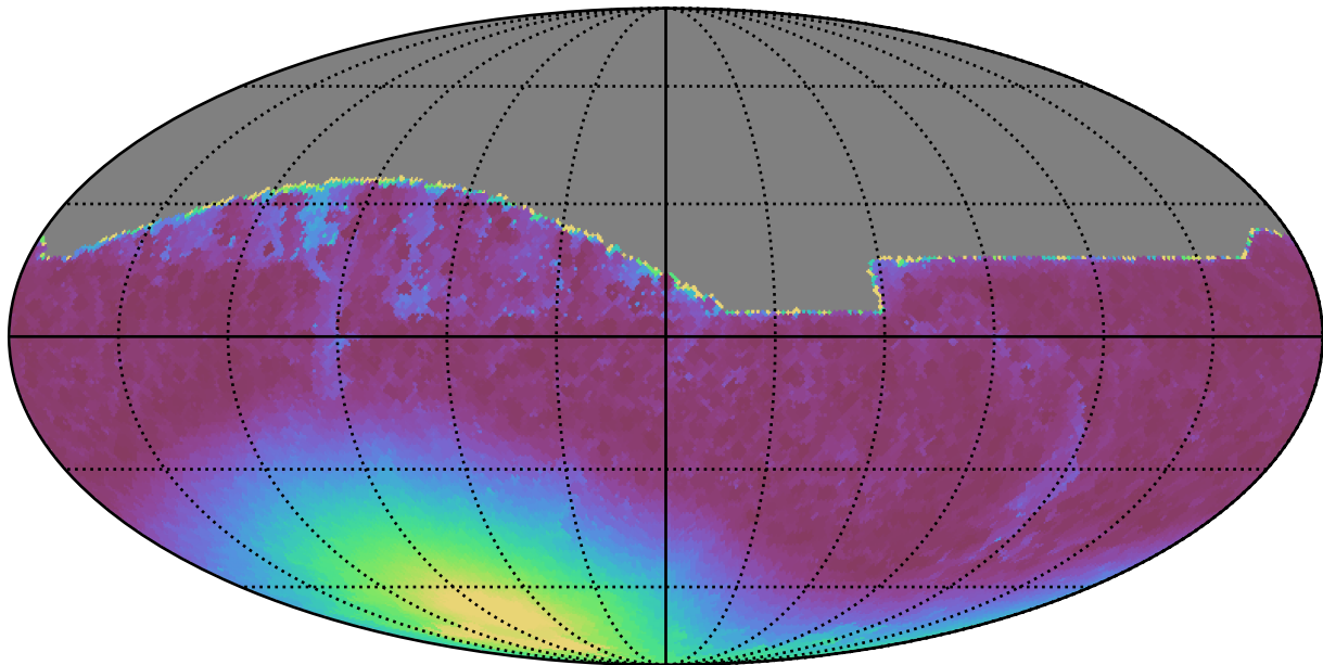
noroll_mjdp365_v3.4_10yrs All sky i band: Min moonDistance
