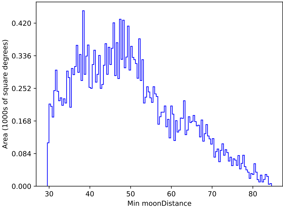
noroll_mjdp365_v3.4_10yrs All sky g band: Min moonDistance
