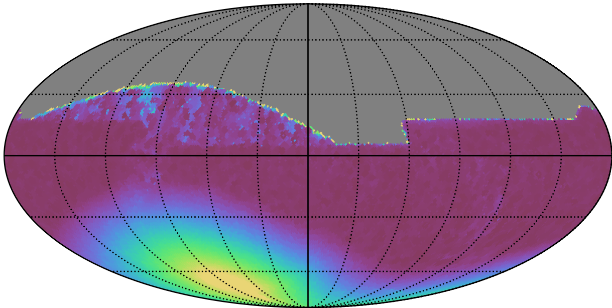
noroll_mjdp365_v3.4_10yrs All sky all bands: Min moonDistance
