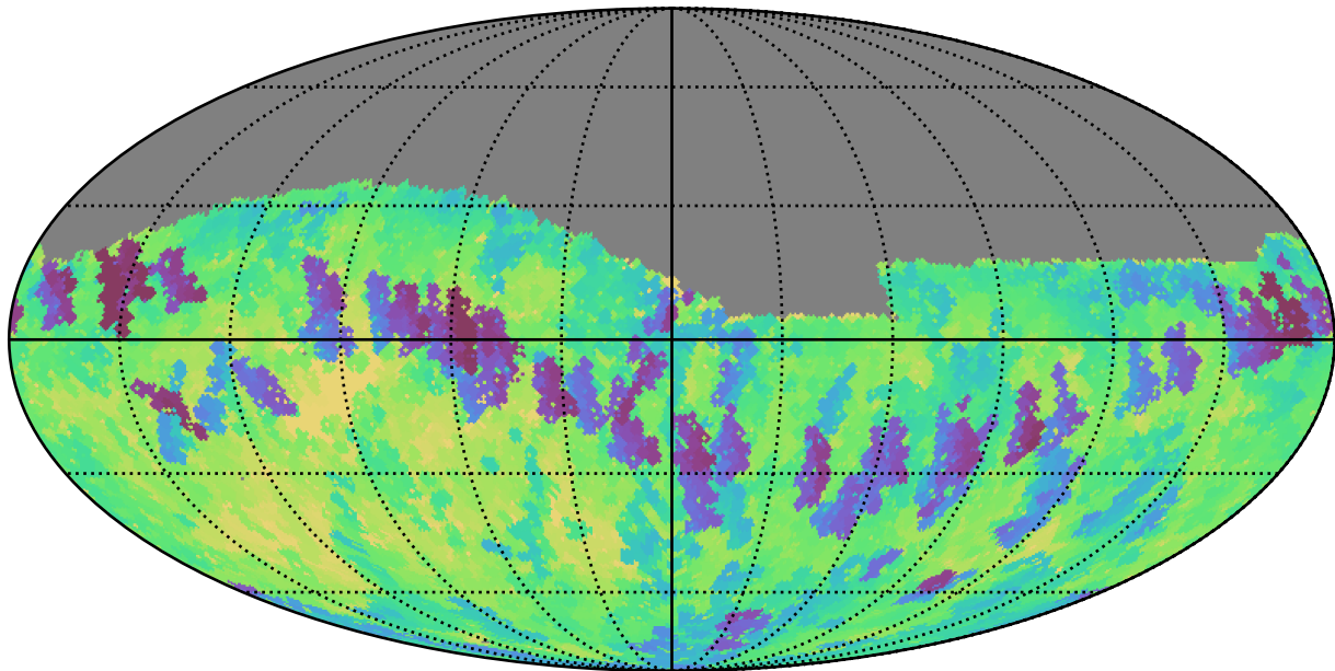
noroll_mjdp365_v3.4_10yrs Yr 1 z band: Min fiveSigmaDepth
