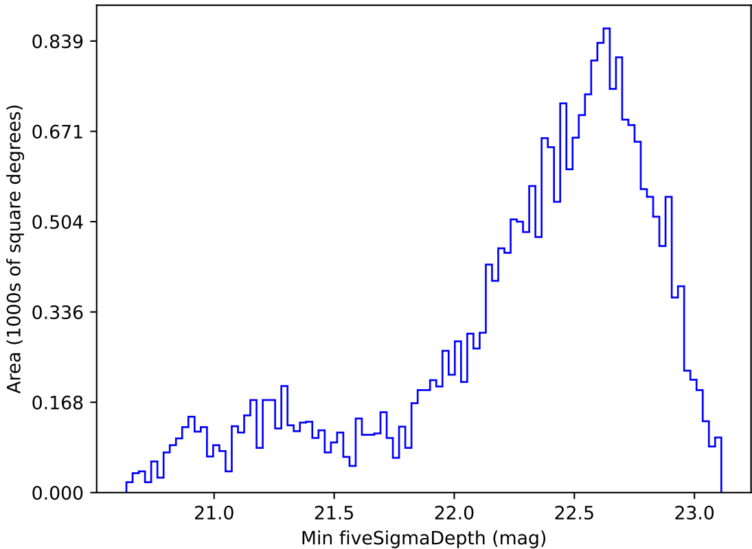
noroll_mjdp365_v3.4_10yrs Yr 1 z band: Min fiveSigmaDepth
