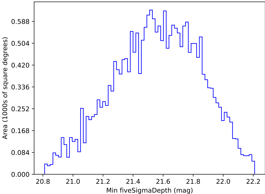
noroll_mjdp365_v3.4_10yrs Yr 1 y band: Min fiveSigmaDepth
