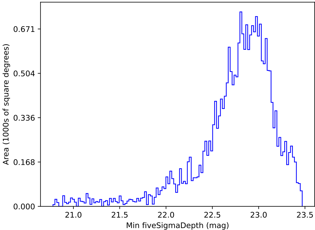
noroll_mjdp365_v3.4_10yrs Yr 1 u band: Min fiveSigmaDepth
