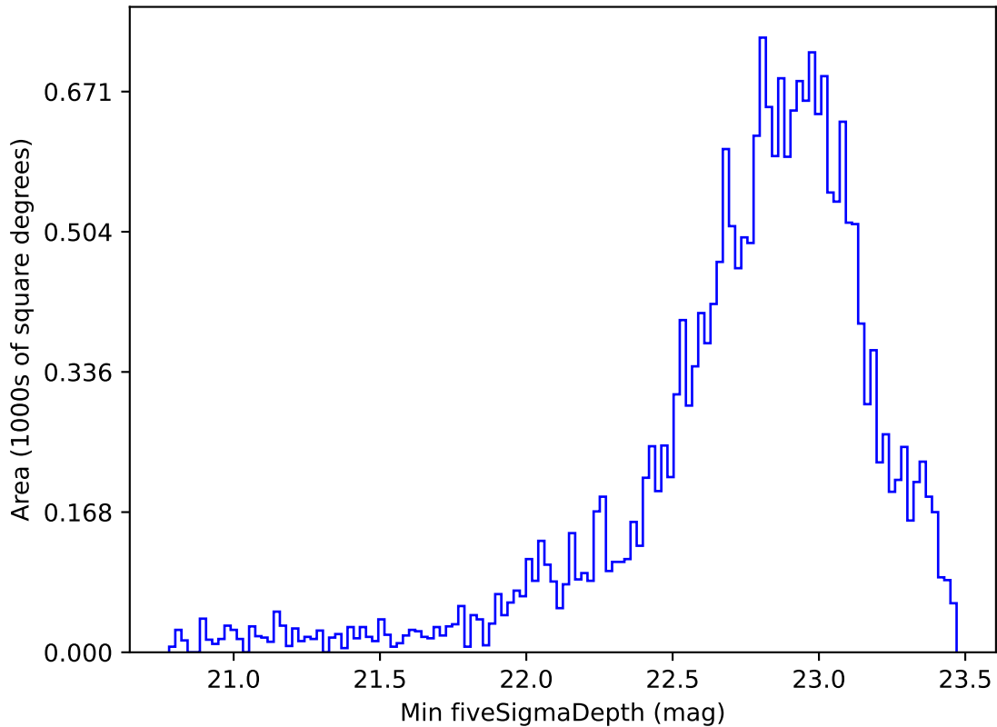
noroll_mjdp365_v3.4_10yrs Yr 1 u band: Min fiveSigmaDepth
