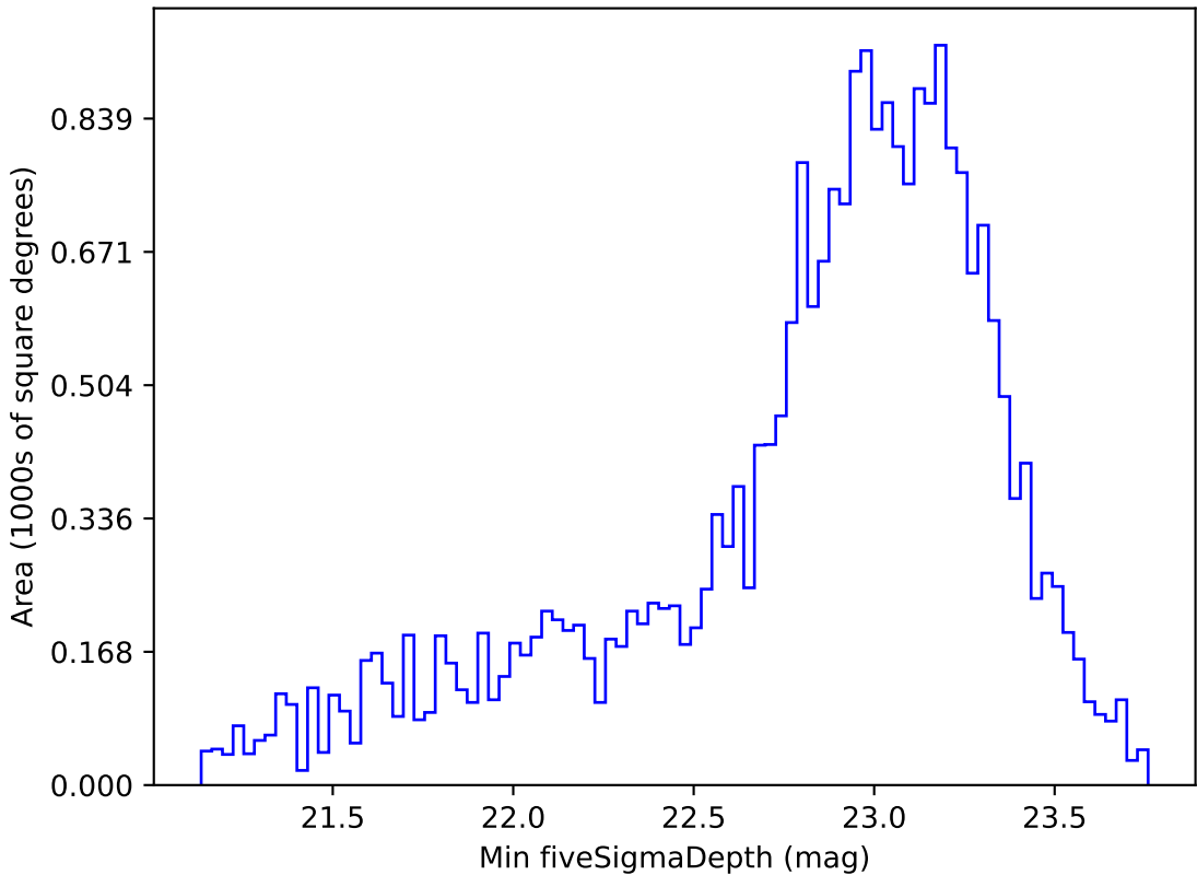
noroll_mjdp365_v3.4_10yrs Yr 1 i band: Min fiveSigmaDepth
