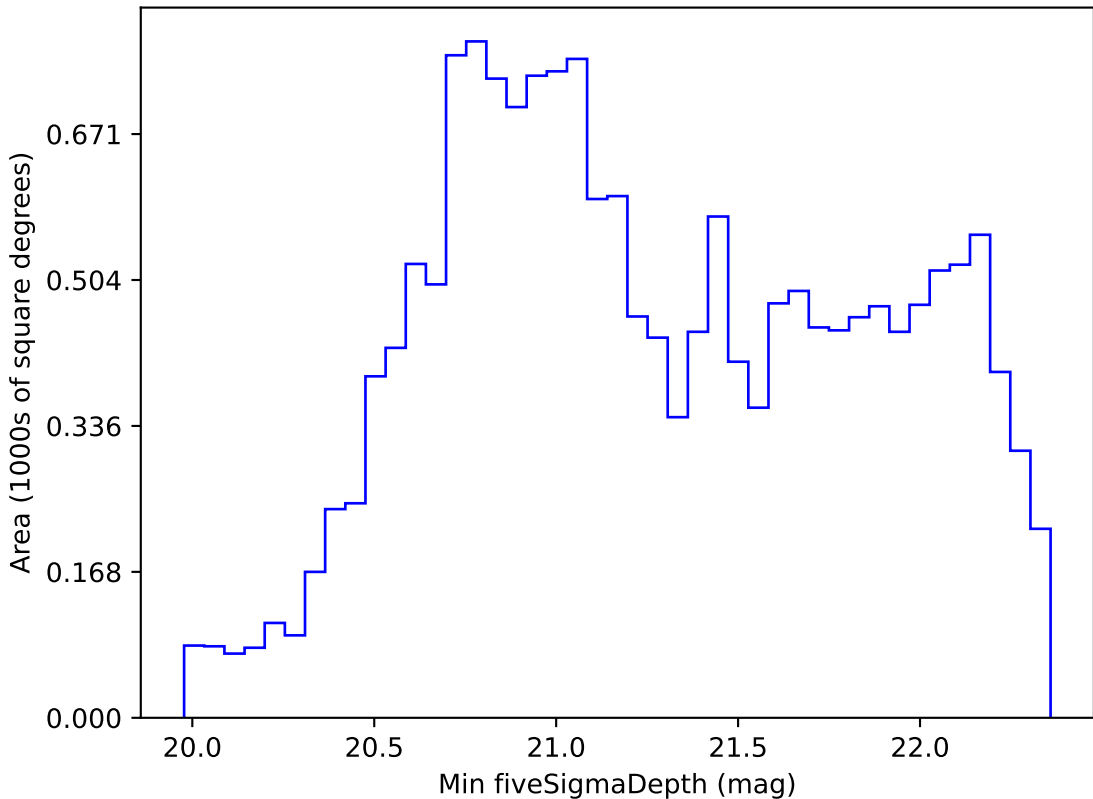
noroll_mjdp365_v3.4_10yrs WFD z band: Min fiveSigmaDepth
