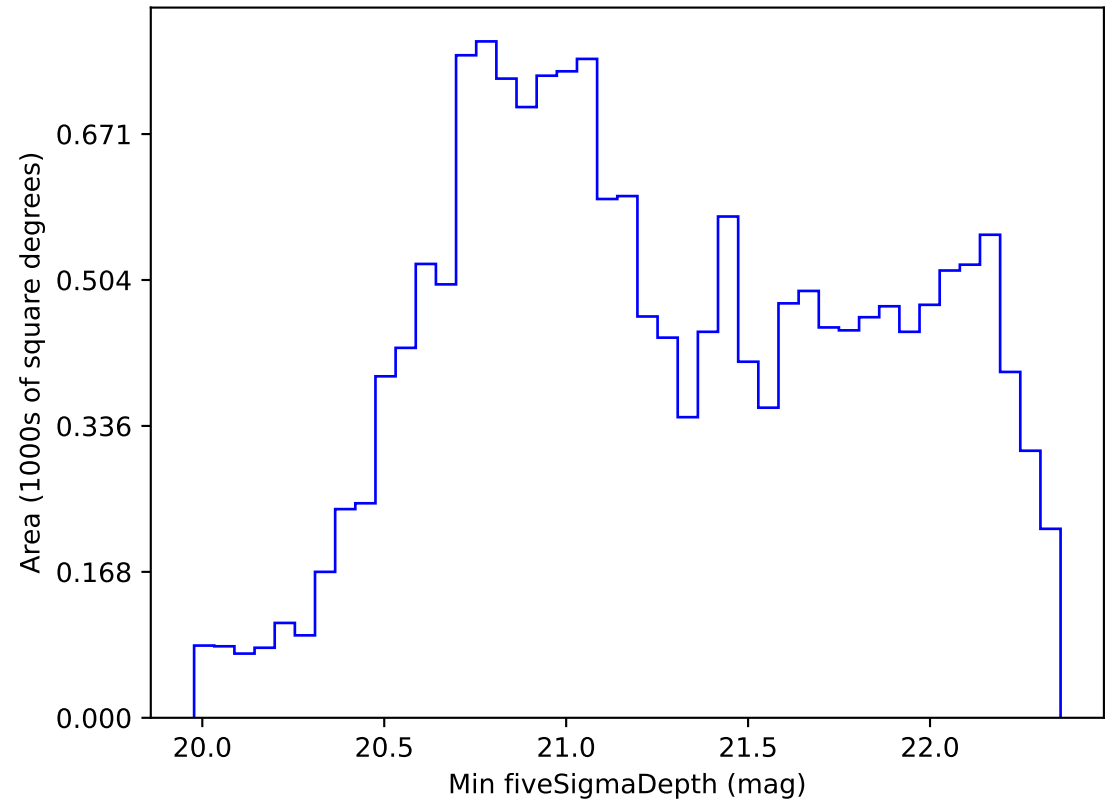
noroll_mjdp365_v3.4_10yrs WFD z band: Min fiveSigmaDepth
