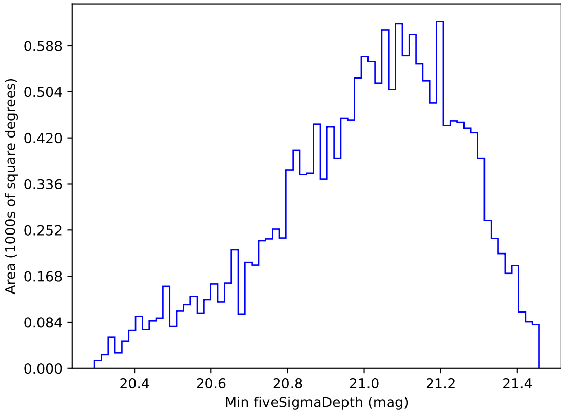
noroll_mjdp365_v3.4_10yrs WFD y band: Min fiveSigmaDepth
