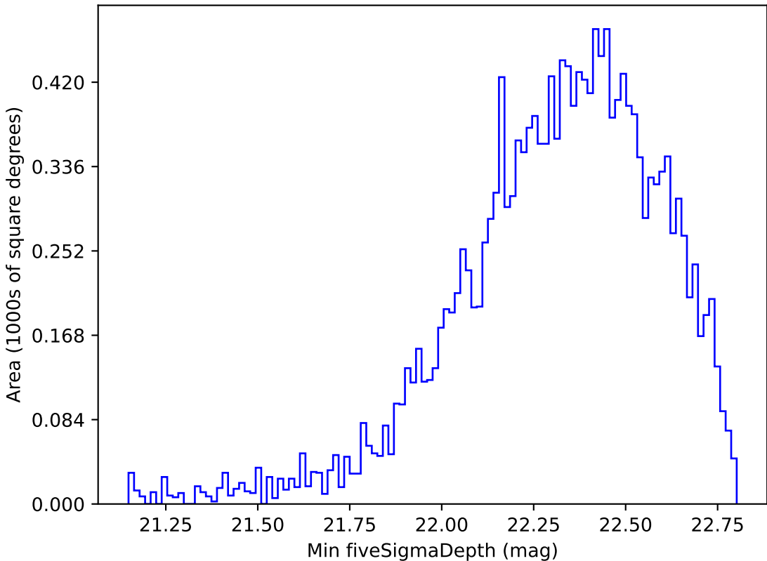
noroll_mjdp365_v3.4_10yrs WFD u band: Min fiveSigmaDepth
