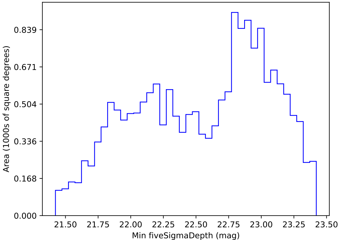
noroll_mjdp365_v3.4_10yrs WFD r band: Min fiveSigmaDepth
