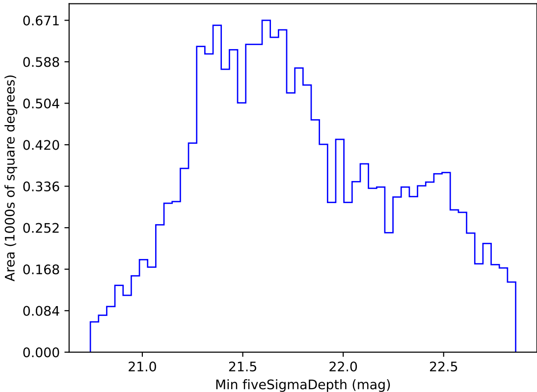
noroll_mjdp365_v3.4_10yrs WFD i band: Min fiveSigmaDepth
