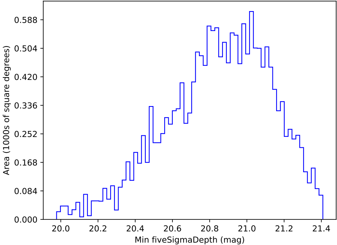
noroll_mjdp365_v3.4_10yrs WFD all bands: Min fiveSigmaDepth
