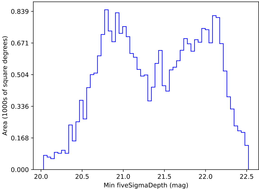
noroll_mjdp365_v3.4_10yrs All sky z band: Min fiveSigmaDepth
