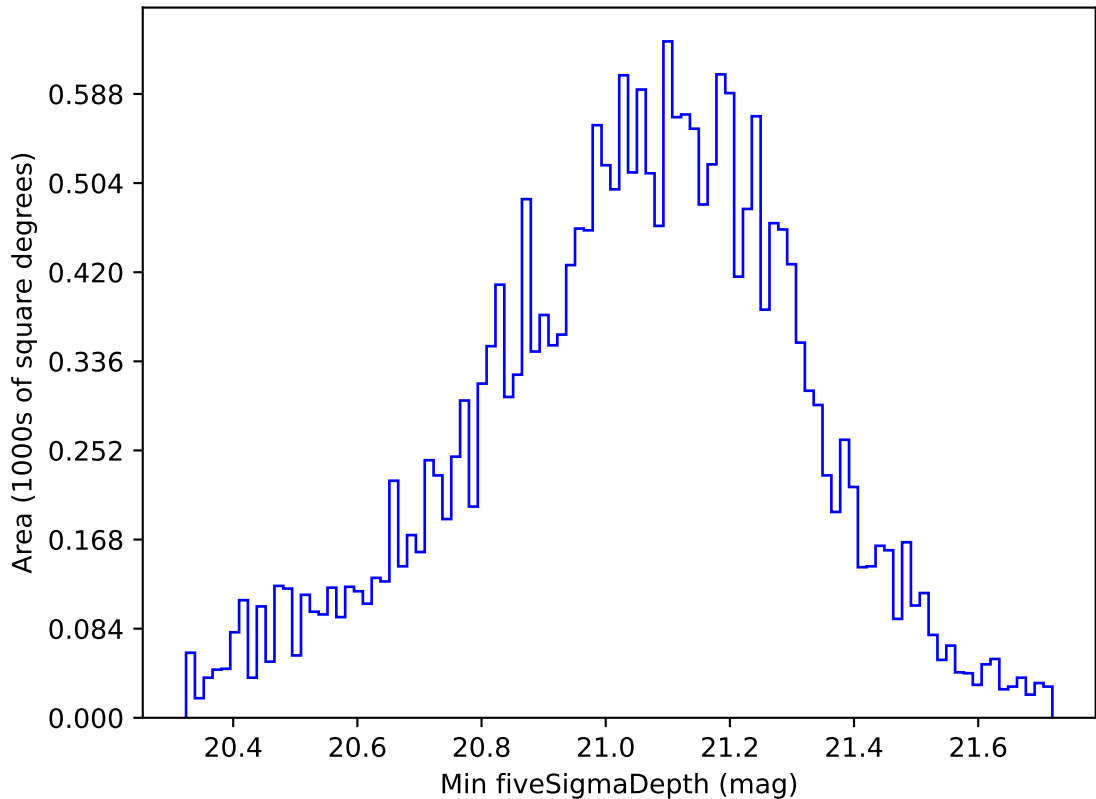
noroll_mjdp365_v3.4_10yrs All sky y band: Min fiveSigmaDepth
