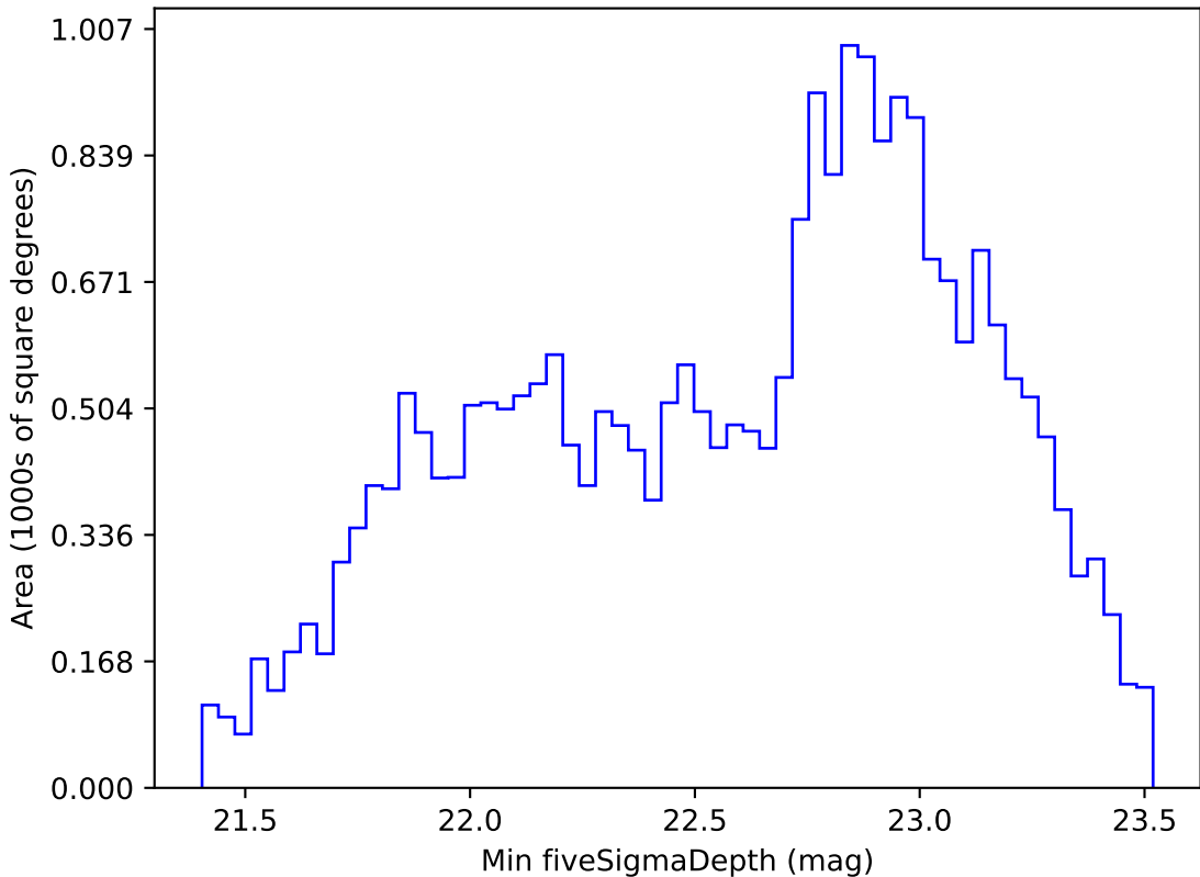
noroll_mjdp365_v3.4_10yrs All sky r band: Min fiveSigmaDepth
