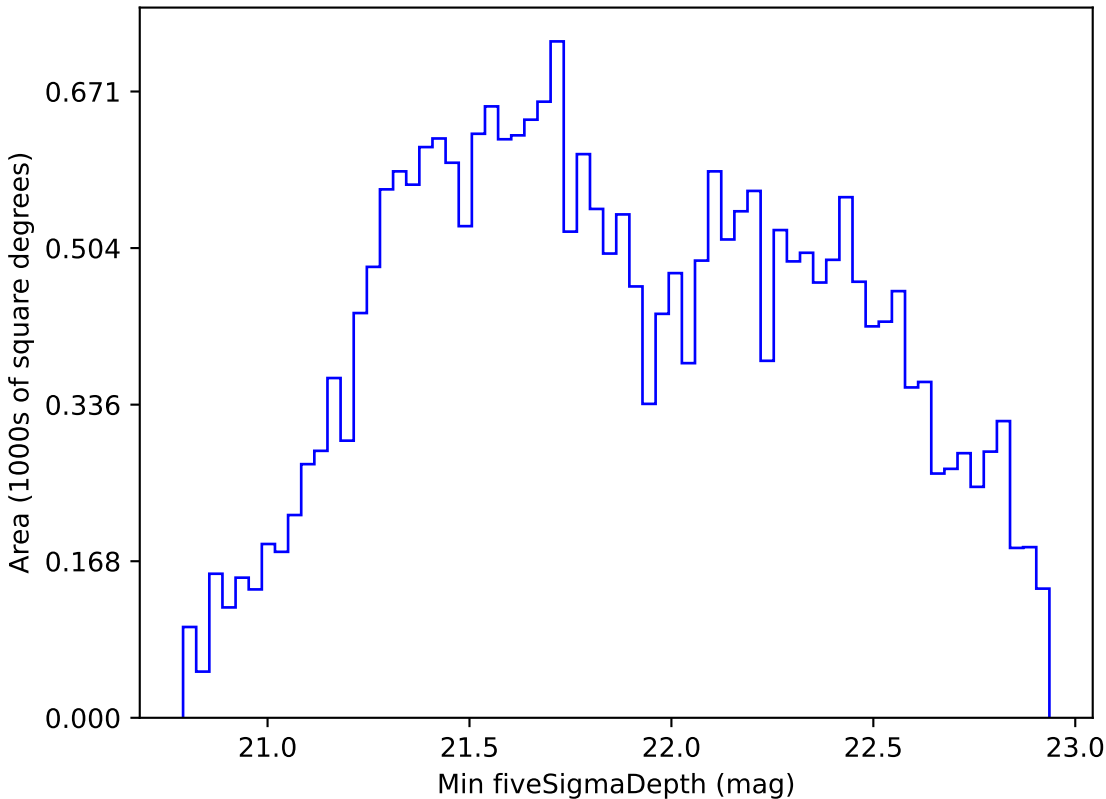
noroll_mjdp365_v3.4_10yrs All sky i band: Min fiveSigmaDepth
