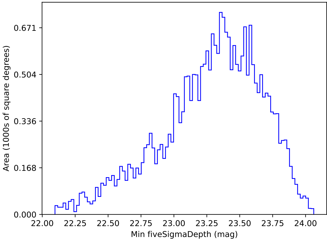
noroll_mjdp365_v3.4_10yrs All sky g band: Min fiveSigmaDepth
