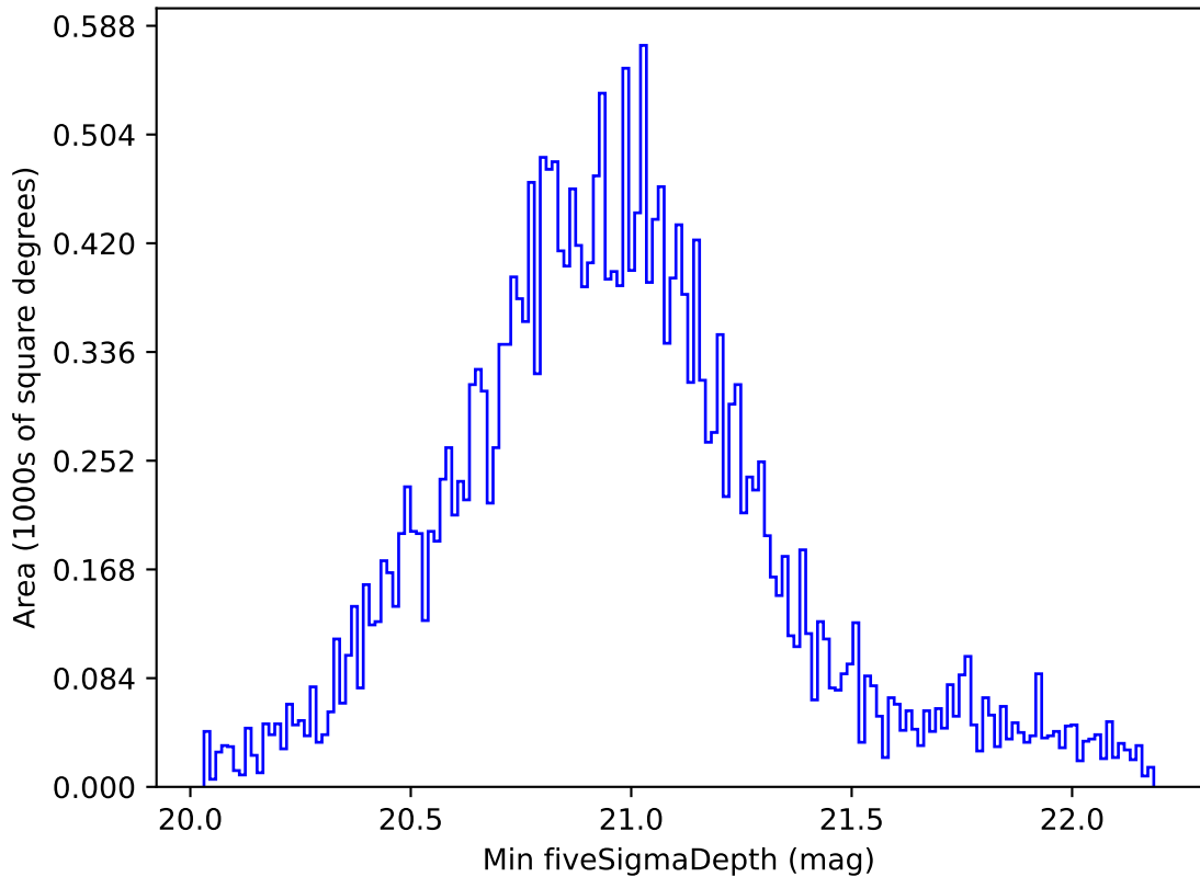
noroll_mjdp365_v3.4_10yrs All sky all bands: Min fiveSigmaDepth
