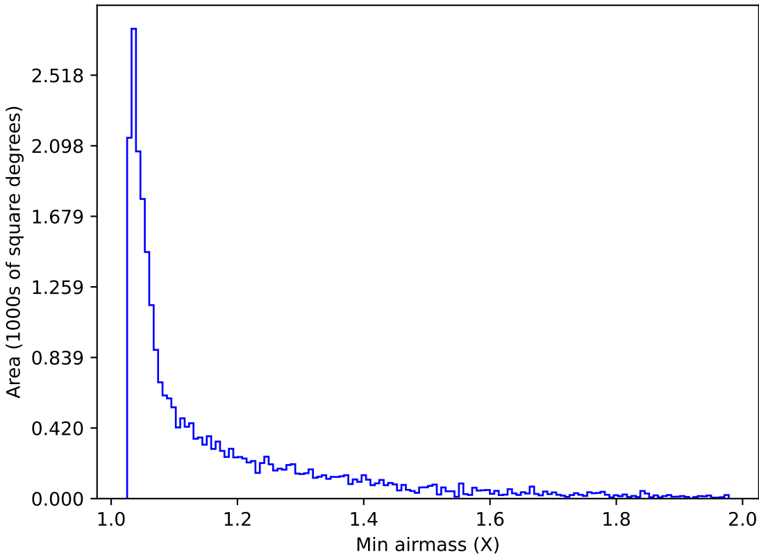
noroll_mjdp365_v3.4_10yrs Yr 1 z band: Min airmass
