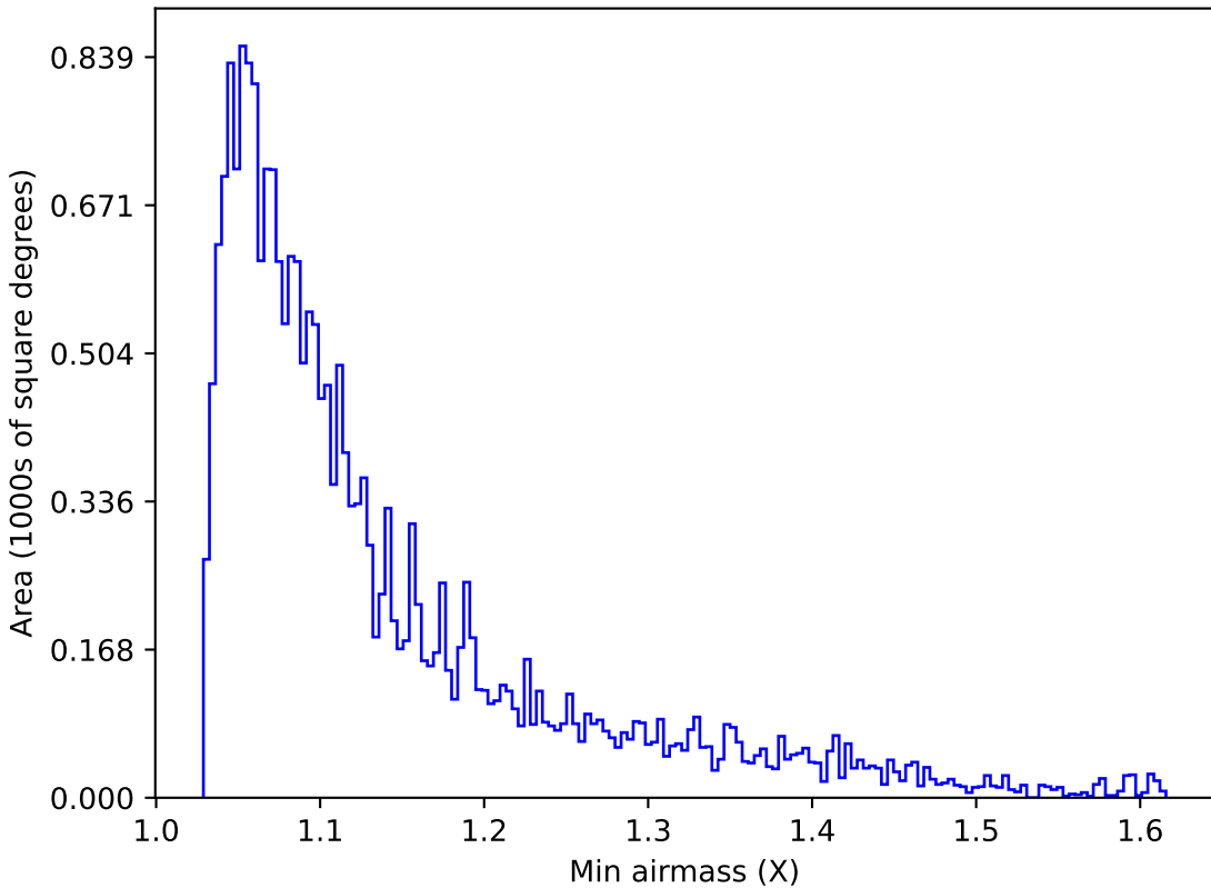
noroll_mjdp365_v3.4_10yrs Yr 1 u band: Min airmass
