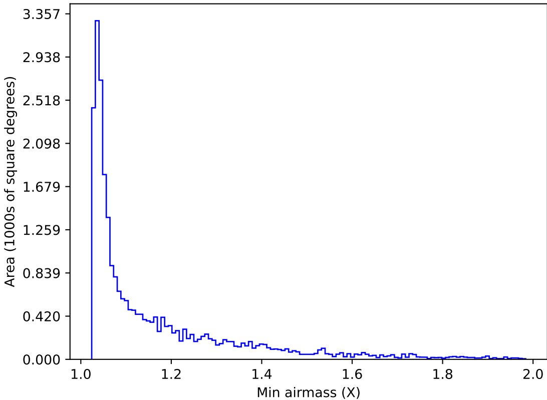
noroll_mjdp365_v3.4_10yrs Yr 1 r band: Min airmass
