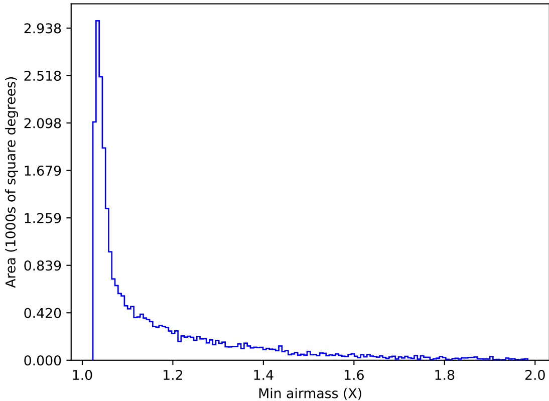
noroll_mjdp365_v3.4_10yrs Yr 1 i band: Min airmass
