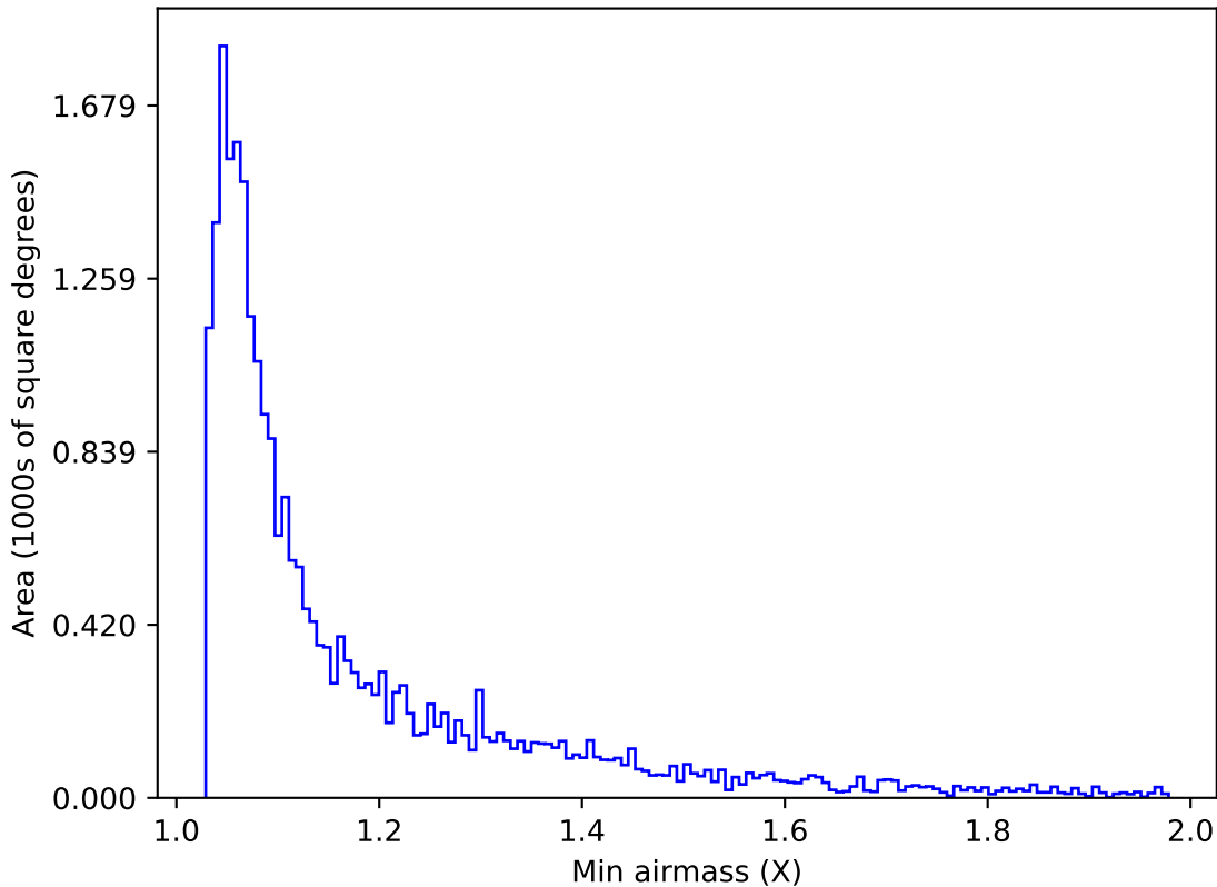
noroll_mjdp365_v3.4_10yrs Yr 1 g band: Min airmass
