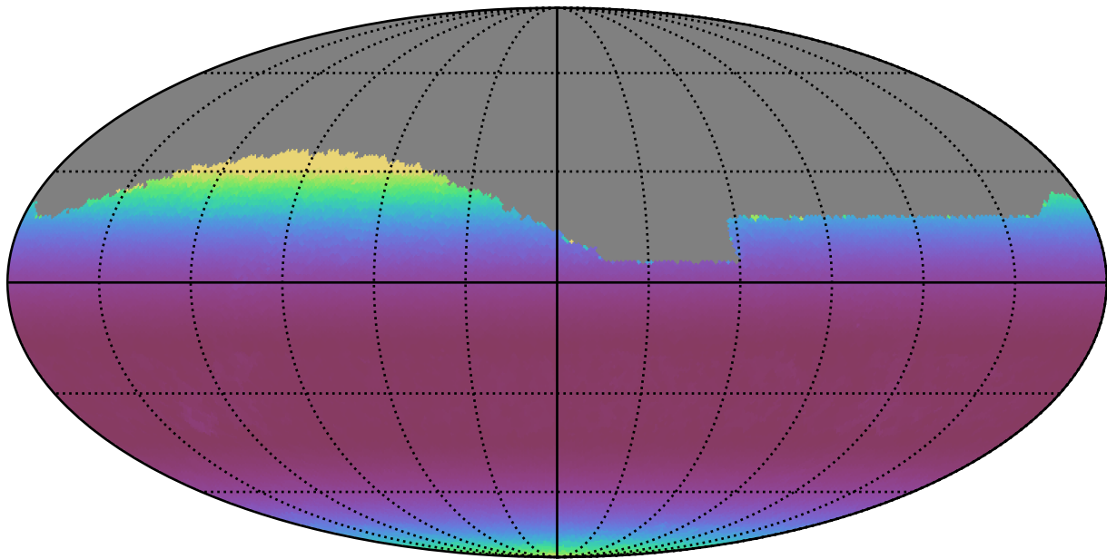
noroll_mjdp365_v3.4_10yrs Yr 1 all bands: Min airmass
