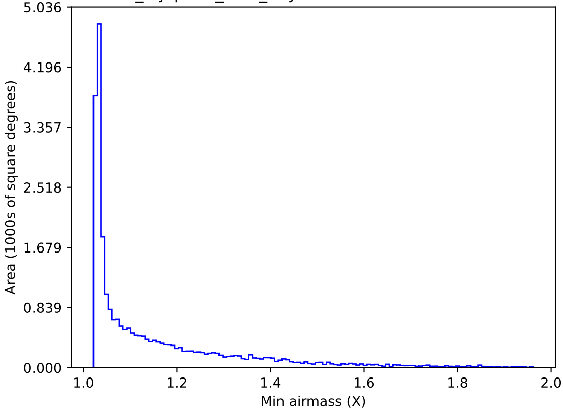
noroll_mjdp365_v3.4_10yrs Yr 1 all bands: Min airmass
