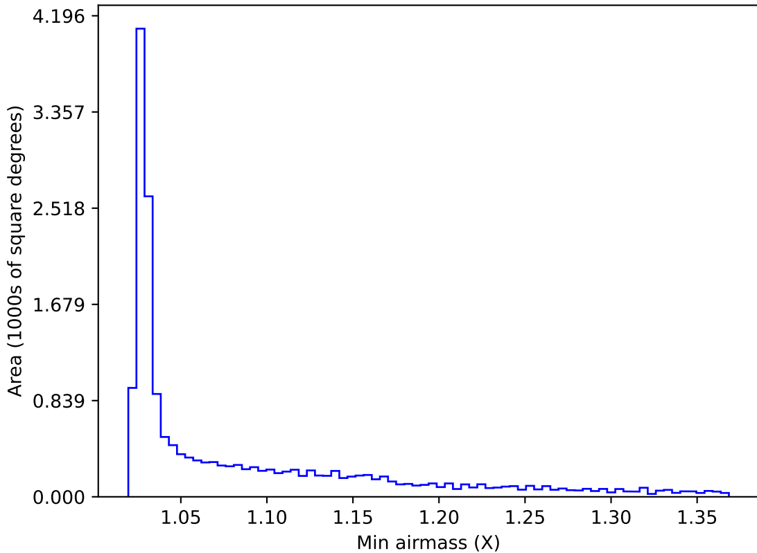
noroll_mjdp365_v3.4_10yrs WFD z band: Min airmass
