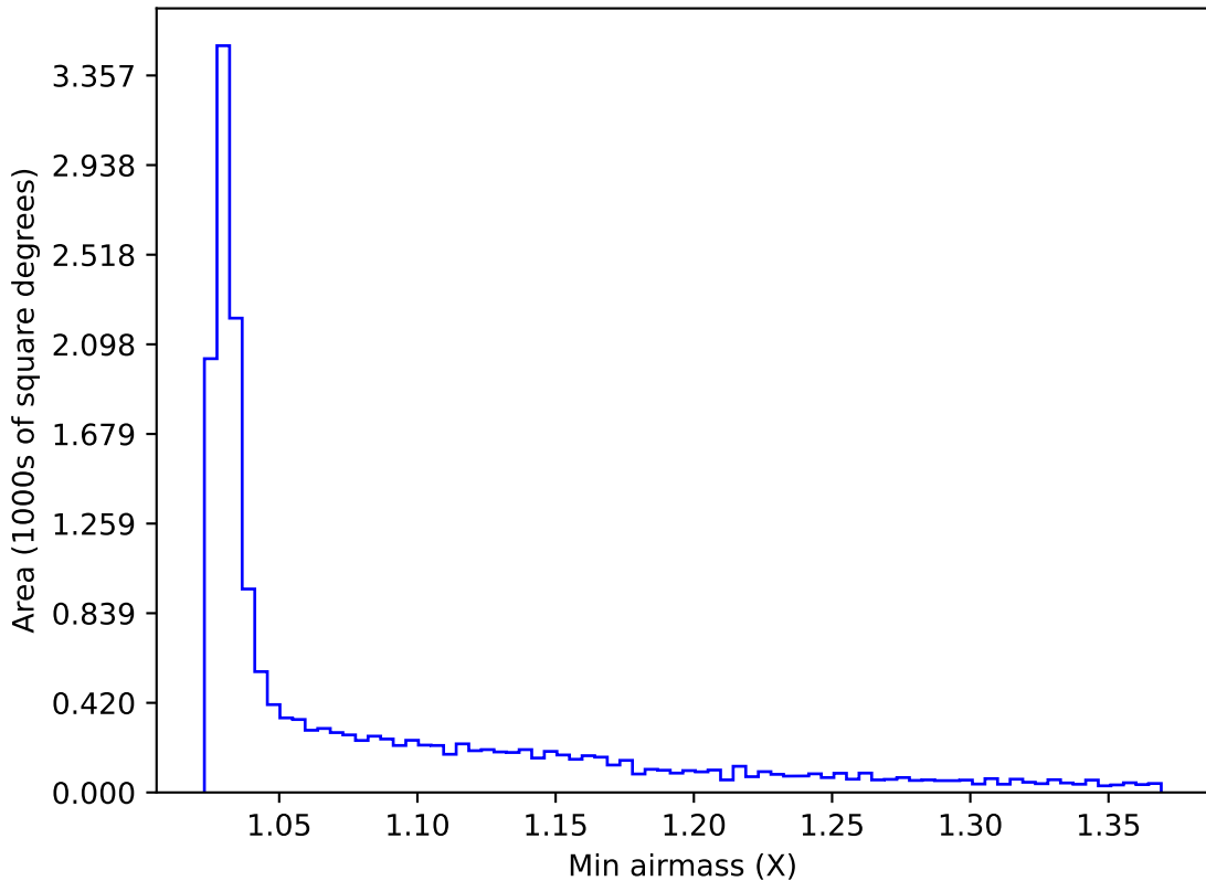
noroll_mjdp365_v3.4_10yrs WFD y band: Min airmass
