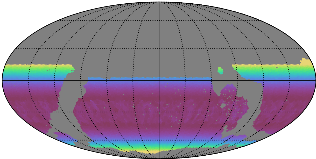
noroll_mjdp365_v3.4_10yrs WFD u band: Min airmass
