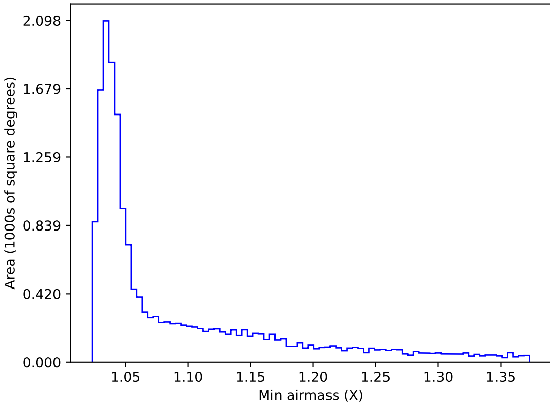
noroll_mjdp365_v3.4_10yrs WFD u band: Min airmass
