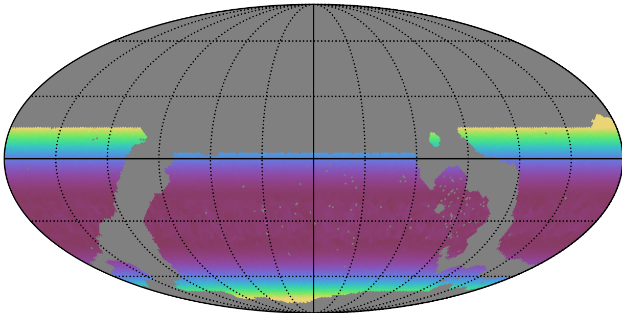
noroll_mjdp365_v3.4_10yrs WFD r band: Min airmass
